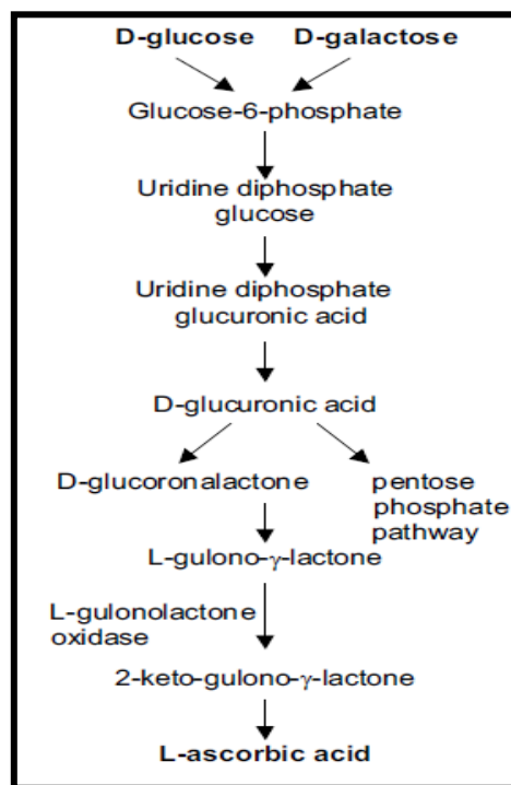
Figure 2: Synthesis Pathway of L-Ascorbic acid
