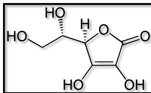
Figure 1: Ascorbic Acid
